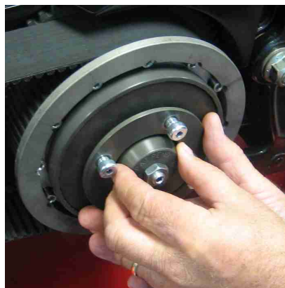
While firmly holding assembly on clutch basket, locate holes in the clutch hub and screw the shoulder bolts in.
